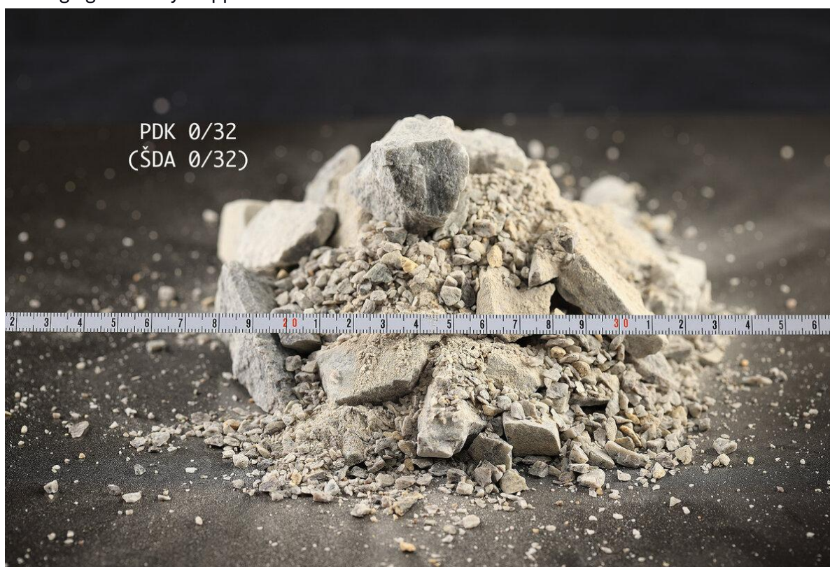
Figure 1 Graded crushed aggregates, PDK 0/32: natural crushed aggregate
