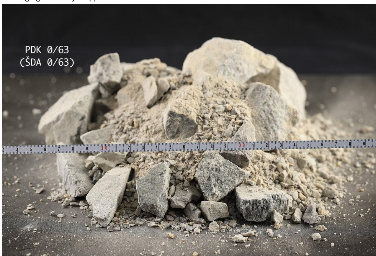
Figure 1 Crushed gravel, PDK 0/63: natural crushed aggregate
